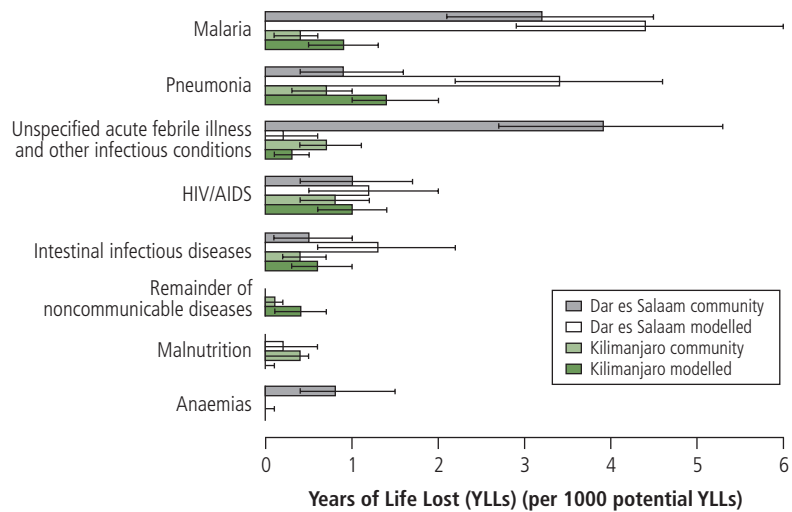
Fig. 2. Comparison of reference and modelled mortality rates in children aged 29 days to 5 years
