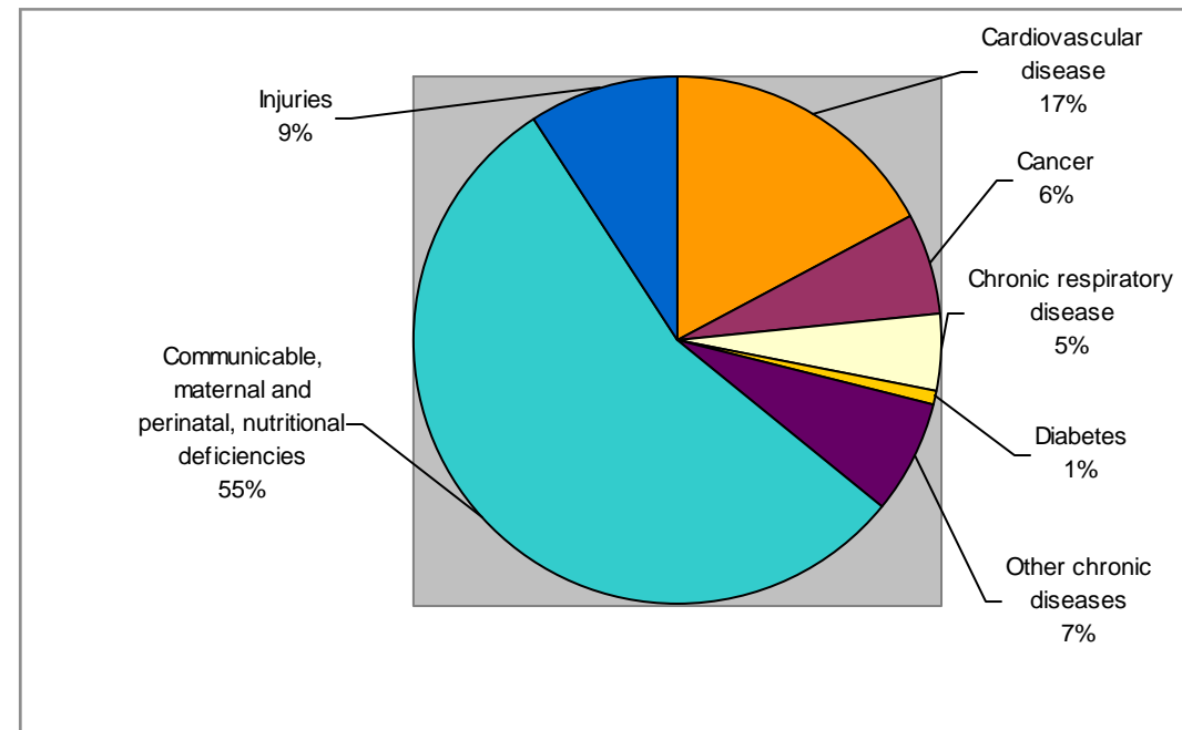
Deaths by cause, all ages, Lao People's Democratic Republic, 2002
