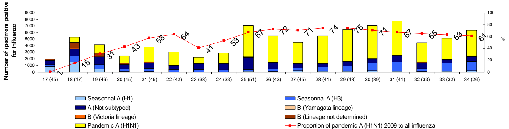
Number of specimens positive for influenza by subtypes (from 19 April to 22 August)
