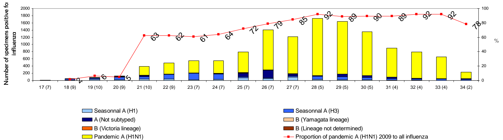
Number of specimens positive for influenza by subtypes (from 19 April to 22 August)
