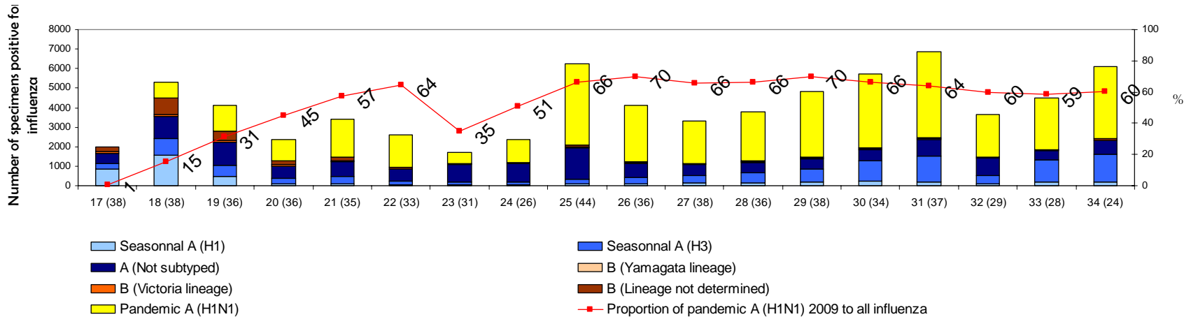
Number of specimens positive for influenza by subtypes (from 19 April to 22 August)
