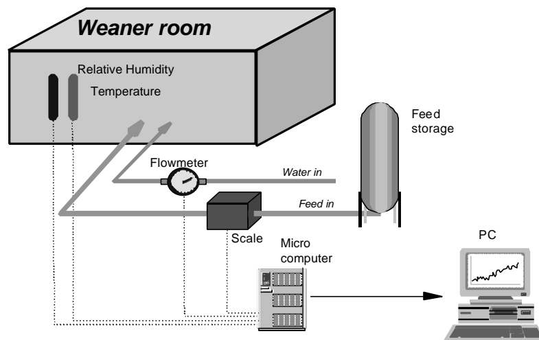
Figure 1. Schematic diagram of experimental set-up.
