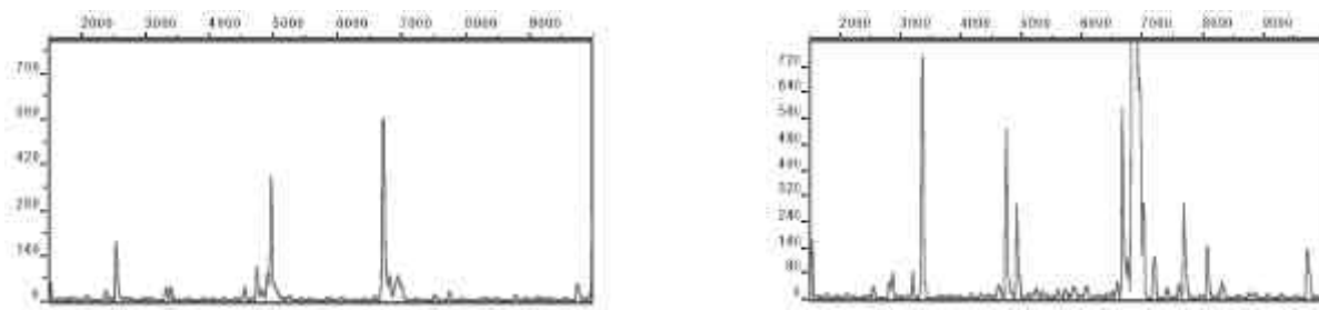
Figure 2. T-RFLP profile from stomach content of pigs fed either fine pelleted feed or coarse meal.
