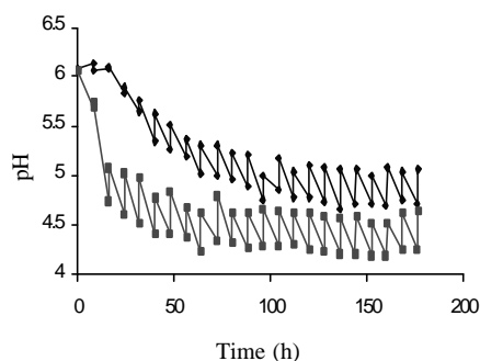
Figure 2. The effect of temperature on pH development during fermentation of liquid feed prepared with eight hours soaking time and 50% residue. -u- 15°C; -g- 25°C. Each point represents the mean value from three fermentations.
