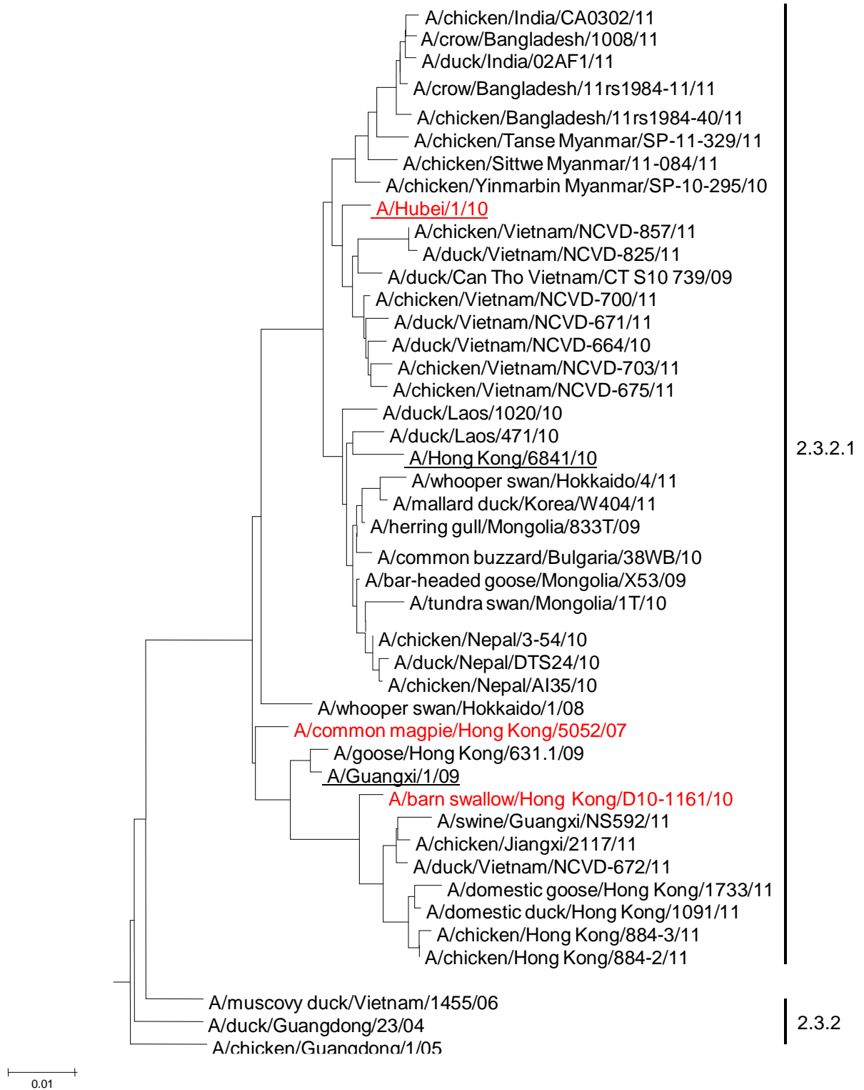
Figure 3. Phylogenetic relationships of A(H5N1) clade 2.3.2, and clade 2.3.2.1 viruses. Vaccine viruses are shown in red. Human viruses are underlined. We gratefully acknowledge the contributions of the originating laboratories and countries that have provided samples and/or submitted sequence data to DDBJ, EMBL-Bank, GenBank, GISAID and other public databases. Sequence data have also been provided by the OFFLU network.
