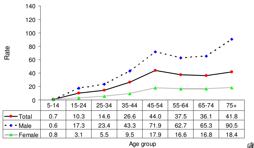
Number of suicides by age group and gender. HUNGARY, 2009.
