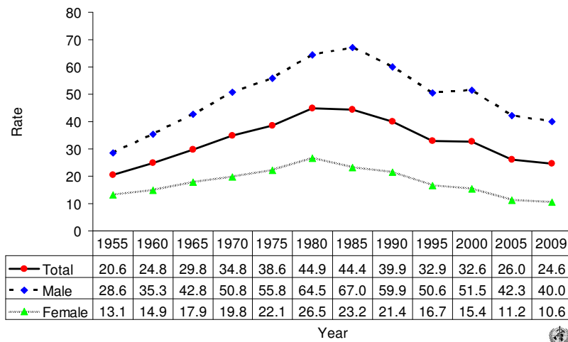
Suicide rates (per 100,000), by gender, Hungary, 1955-2009.
