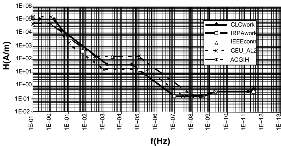
Figure 2. Comparison of magnetic field strength limit values for workers and continuous exposure over a full working day (for notations see box). Details as in Figure 1.
