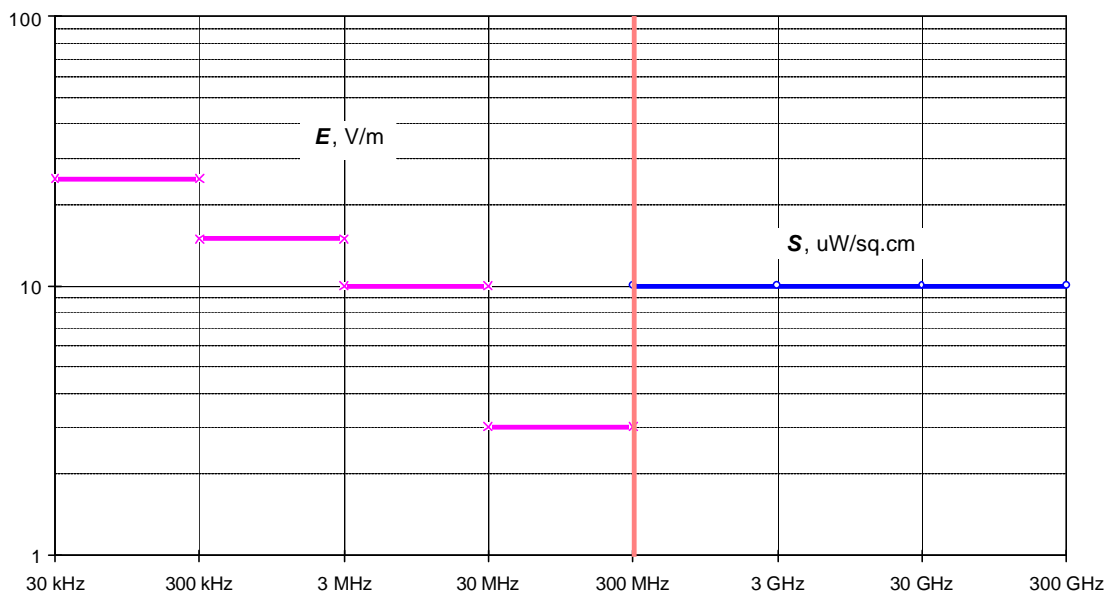
Fig. 4. Limit values for electric field strength E and power flux density S (public areas) according to SanPiN 2.2.4/2.1.8.055-96
