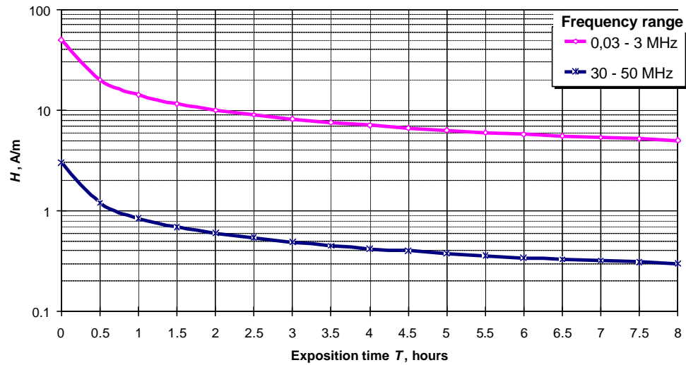
Fig. 2. Limit values for magnetic field strength H (workplace) according to GOST 12.1.006-84 and SanPiN 2.2.4/2.1.8.055-96
