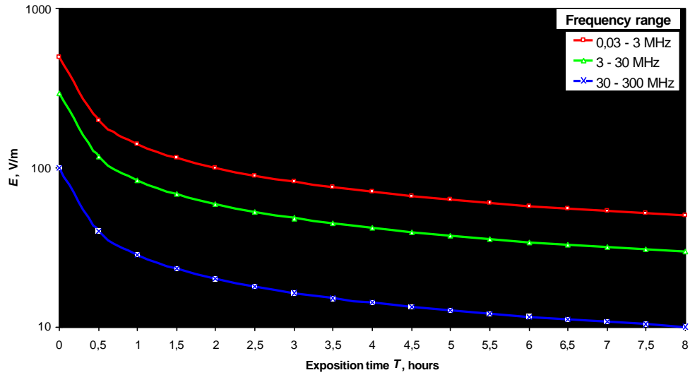
Fig. 1 Limit values for electric field strength E (workplace) according to GOST 12.1.006-84 and SanPiN 2.2.4/2.1.8.055-96
