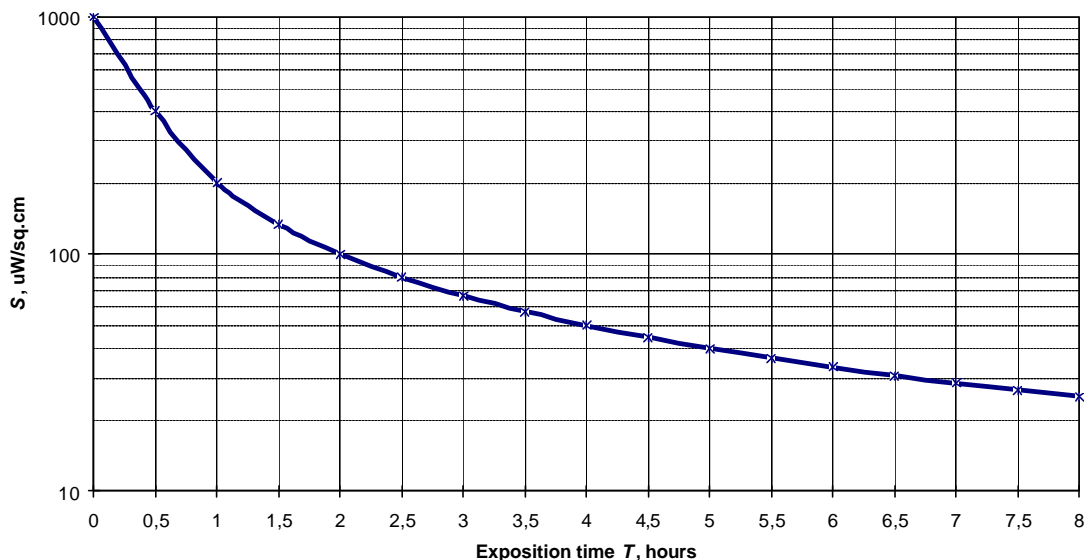
Fig. 3. Limit values for power flux density S in the frequency range 0,3 - 300 GHz (workplace) according to GOST 12.1.006-84 and SanPiN 2.2.4/2.1.8.055-96
