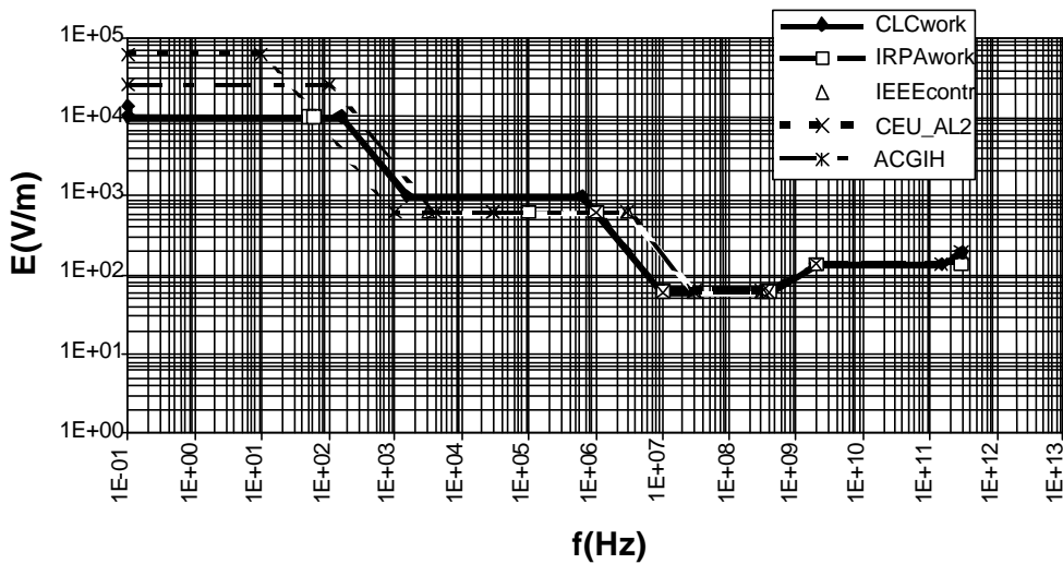
Figure 1. Comparison of electric field strength limit values for workers and continuous exposure over a full working day (for notations see box). CENELEC set reference levels over the entire frequency range. IRPA limit values exist at 50/60 Hz and in the frequency range 100 kHz to 300 GHz. The medium action level of CEU is denoted by CEU AL2. The IEEE limit values are defined in the frequency range from 3 kHz to 300 MHz and refer to controlled areas. They coincide with ACGIH's threshold limit values for workers which extend to lower frequencies. For higher frequencies power density limit values are set by these American institutions.
