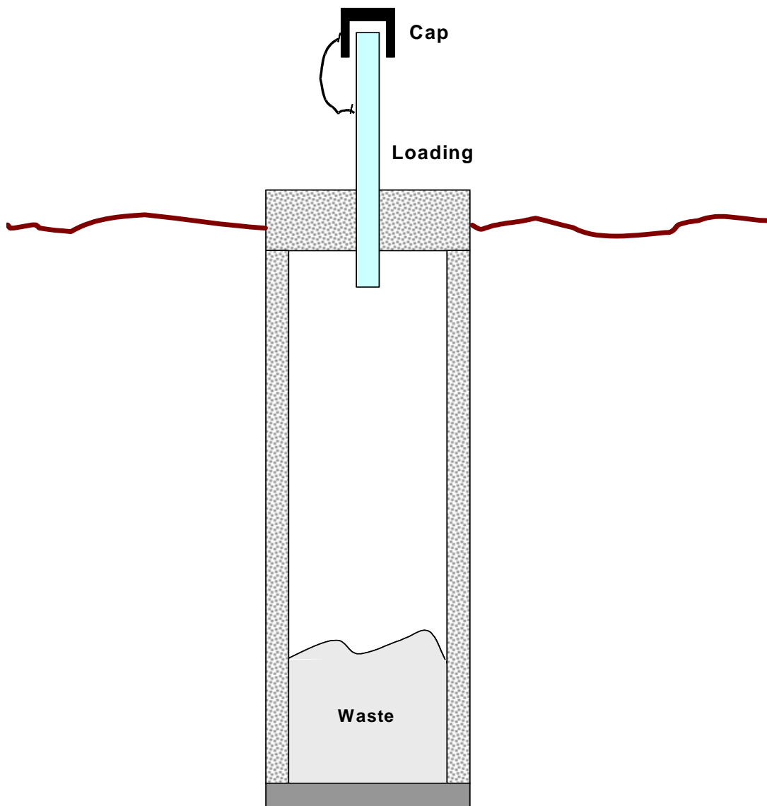
Figure E1. Cross - sectional view of secured disposal pit for sharps
